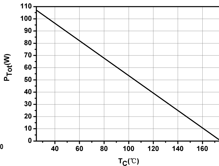
Fig.6-Power Derating
