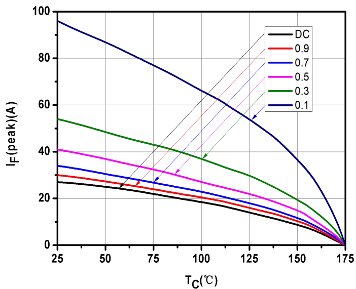
Fig.7-Current Derating
